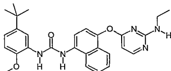
1-(5-tert-Butyl-2-methoxy-phenyl)-3-[4-(2-ethylamino-pyrimidin-4-yloxy)-naphthalen-1-yl]-urea;
